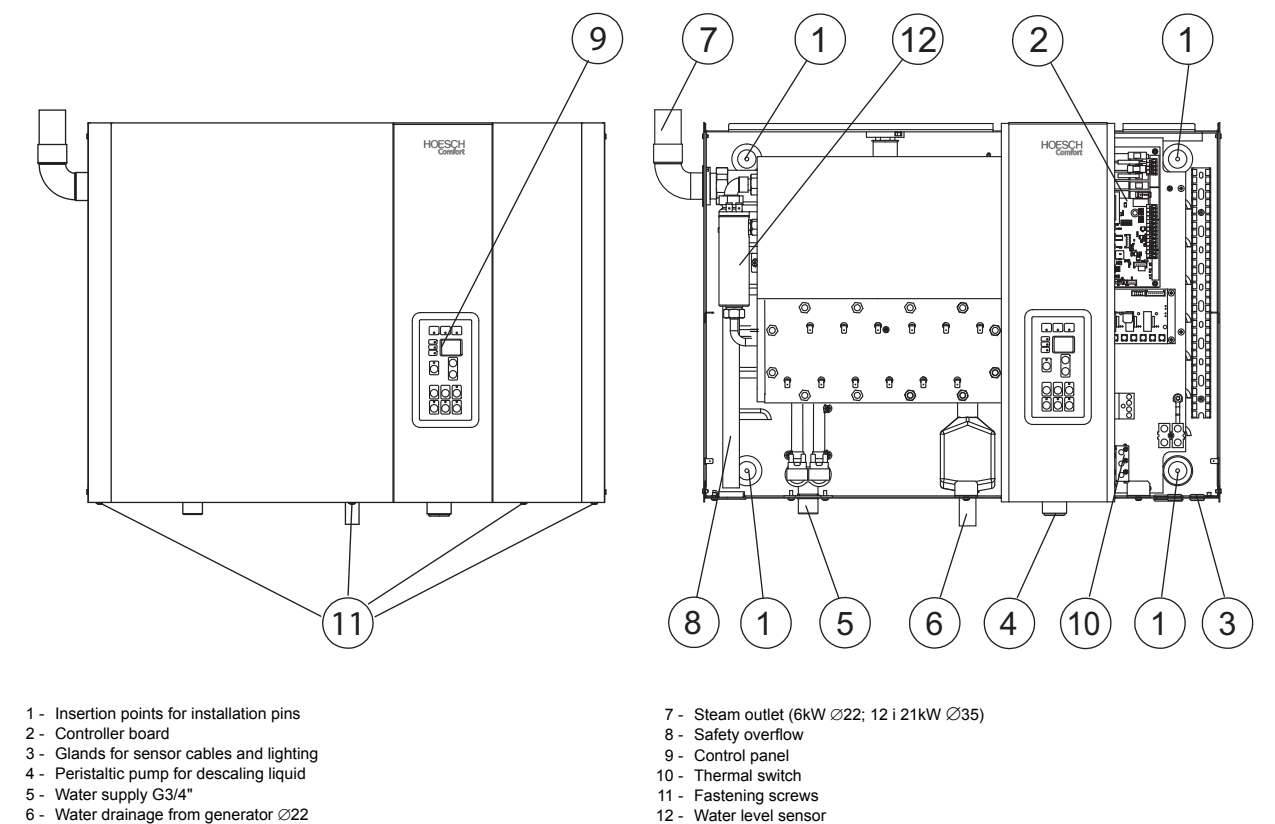
Fig. 1 Structure of steam generator
