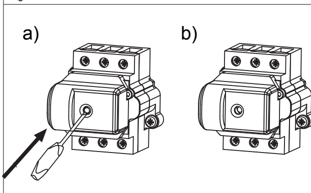
Fig.4.4 Schakelaar WT3a
