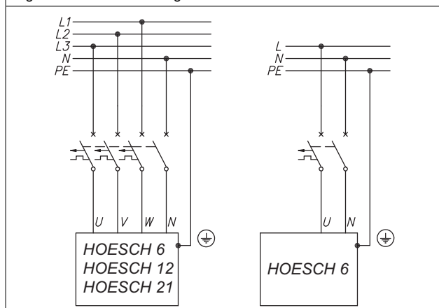
Fig. 4.1 Connection diagram
