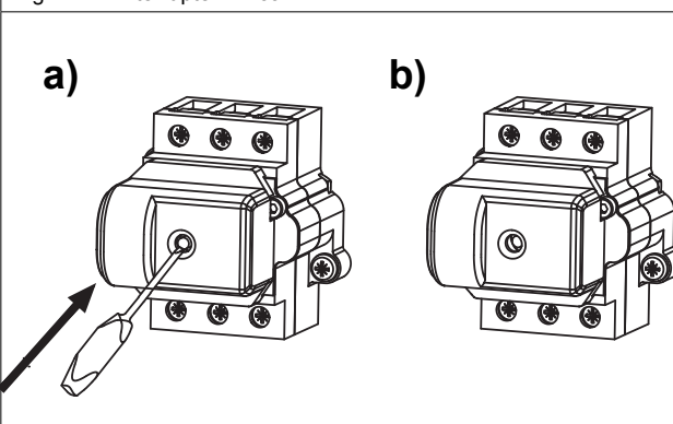
Fig. 4.4 Interrupter WT3a
