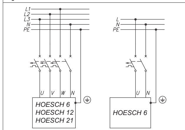
Figure 4.1 Schéma de raccordement
